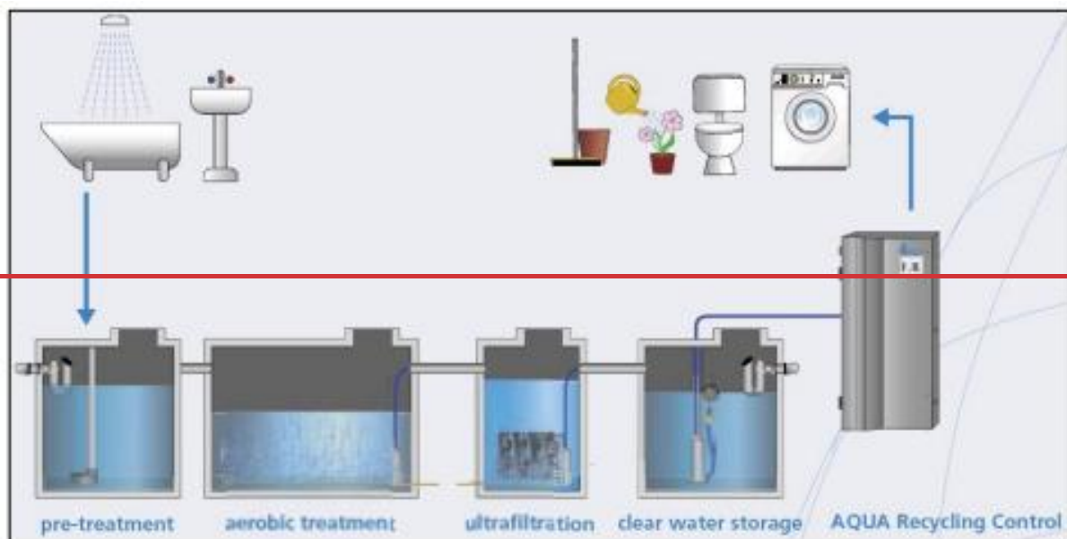
Figure 32: A typical domestic greywater recycling system 20
